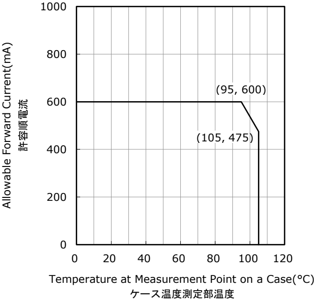
Temperature at Measurement Point on a Case vs Allowable Forward Current
